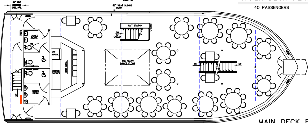
MAIN DECK PLAN 106 PASSENGERS
